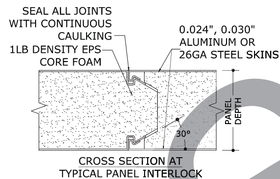
2 PANEL INTERLOCK DETAIL 1 N.T.S. DETAIL
