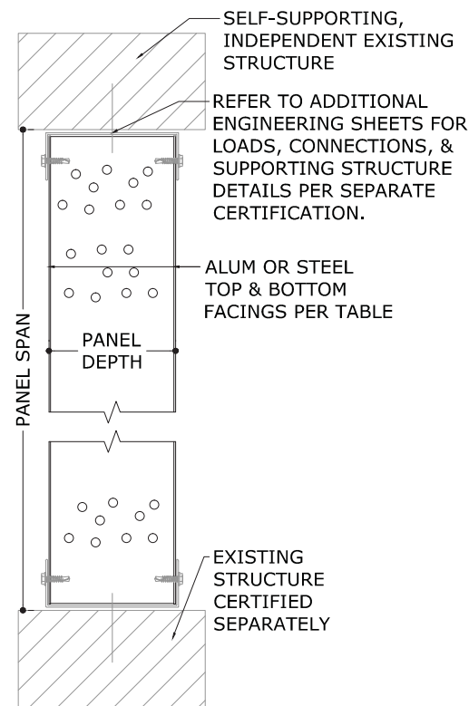
1 WALL PANEL SPAN 1 N.T.S. PLAN OR SECTION
